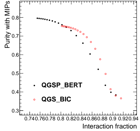
(b) Fcut optimization at 2 GeV with fixed Ecut. (Ecut = 3 MIPs)
