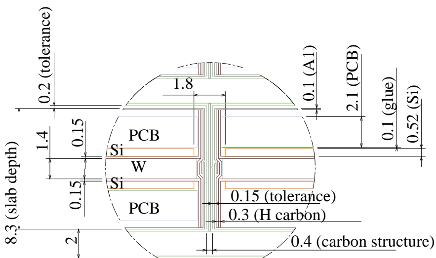
(b) Detailed transverse view of a slab. One passive tungsten layer is sandwiched between two active silicon layers. The upper silicon layer is preceded by a large amount of passive material (glue, the PCB, aluminum, the carbon structure as well as a tungsten layer), the lower one only by one tungsten layer. Dimensions are in mm.
