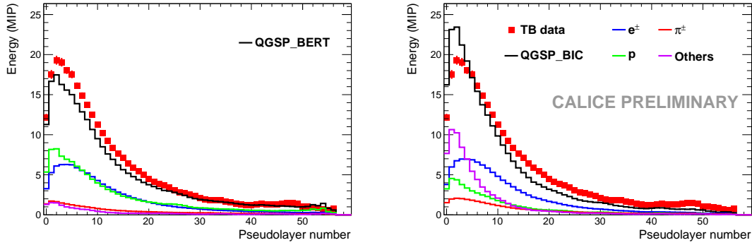
(a) BERT : valid for QGSP_BERT (shown here) and FTFP_BERT (b) LEP : valid for QGSP_BIC (shown here), QGS_BIC and LHEP
