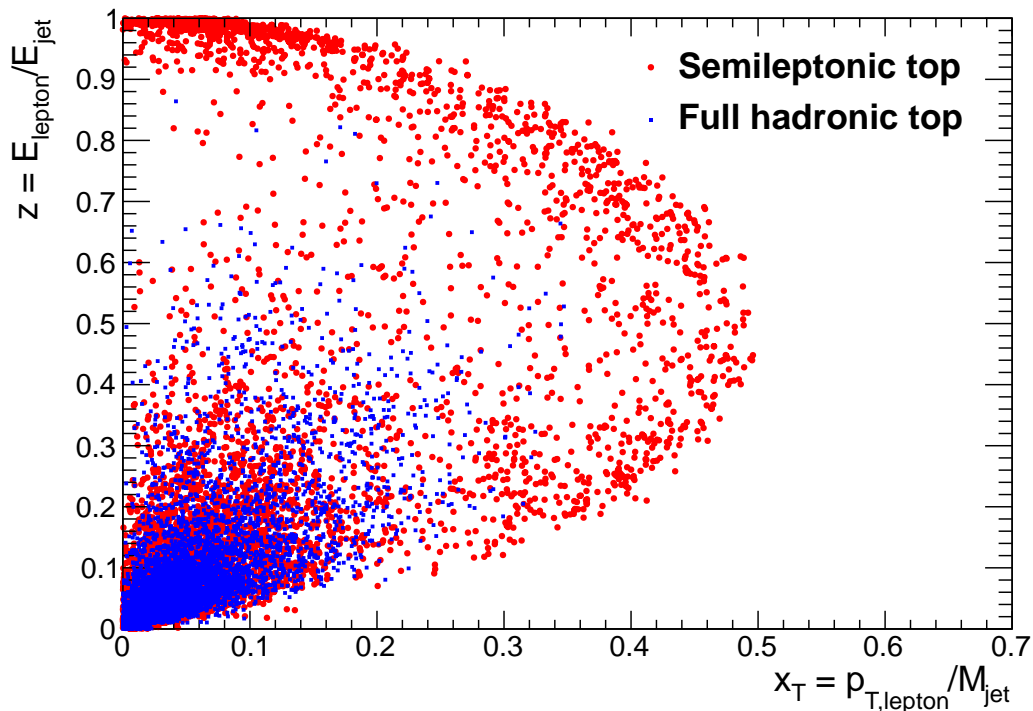
Figure 11.3: Isolation variables applied to a sample of leptons from semileptonic (red) and full hadronic (blue) top events. Isolated leptons and leptons from the decays of bottom mesons are identified and separated.
