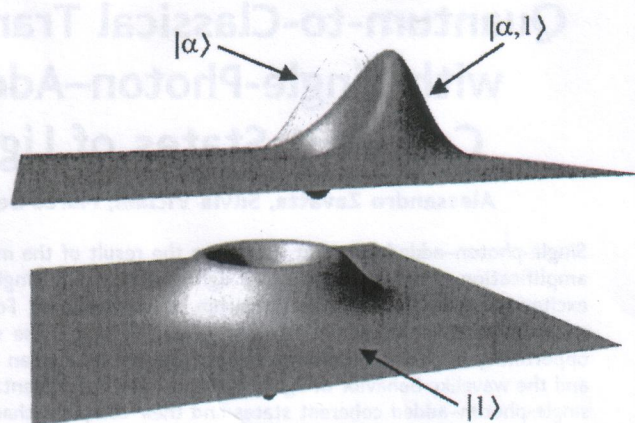
Fig. 1. Theoretical Wigner functions for some of the quantum states of light discussed in the text. Upper surface, SPACS |\alpha, 1\rangle ; wire-frame surface, original unexcited coherent state |\alpha\rangle ; lower surface, single-photon Fock state |1\rangle . The horizontal plane coordinates represent two orthogonal quadratures of the field. The single-photon Wigner function is centered at the origin of the phase space. A value of |\alpha|^2 = 1 is used.
