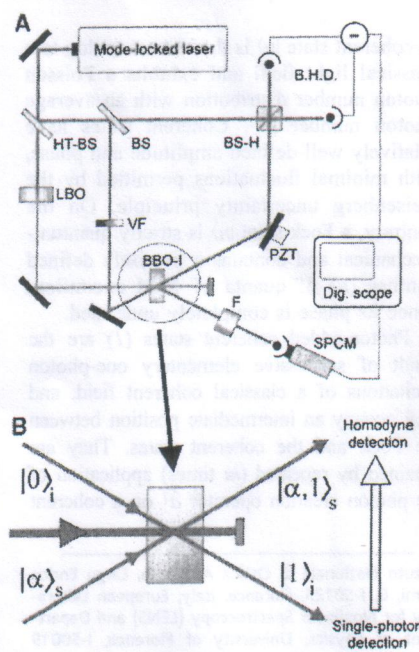
Fig. 2. Experimental apparatus and conceptual scheme for the conditional SPACS preparation.
