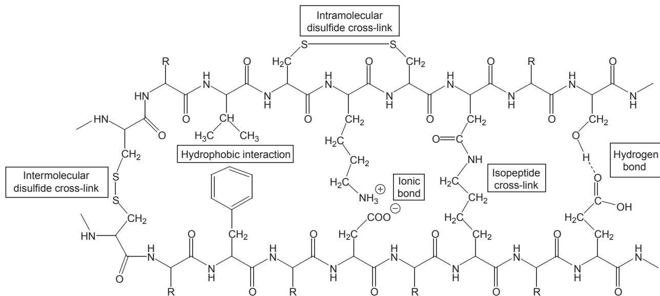
Figure 8.1 Covalent bonds and non-covalent interactions in wool.
