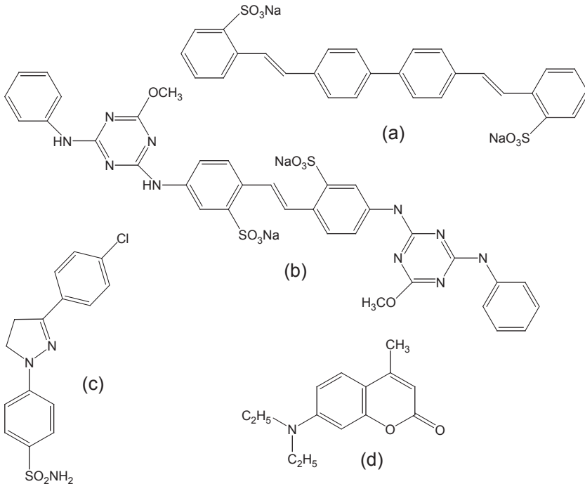
Figure 8.18 Chemical structure of common FWAs. (a) Uvitex NFW (distyrylbiaryl), (b) Uvitex CF (stilbene), (c) Blankophor DCB (pyrazoline) and (d) 7-diethylamino-4-methylcoumarin.
