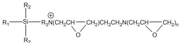
Figure 8.21 Chemical structure of water-soluble epoxide for cross-linking silk ( R_1 , R_2 , R_3 are alkyl groups and n = 1 or 2 ).
