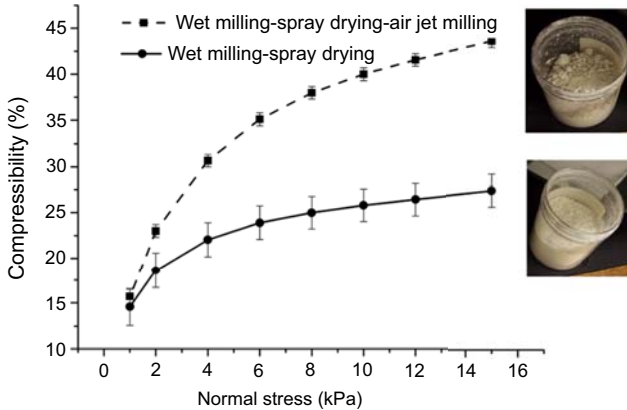
Figure 16.11 Compressibility of wool powder.
