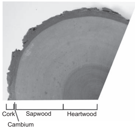
Figure 18.2 Cross-section (transversal view) of a tree trunk.
