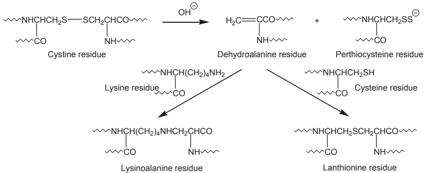
Figure 8.12 Formation of lantionine and lysinoalanine cross-links during the permanent setting of wool.
