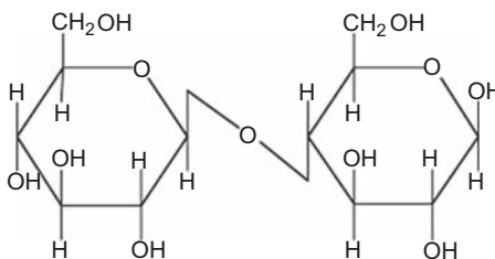
Figure 1.10 D-Glucopyranose units.
