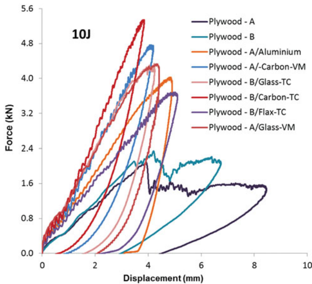
Figure 2. Typical load displacement curves for 10 J impacts for the eight configurations tested.
