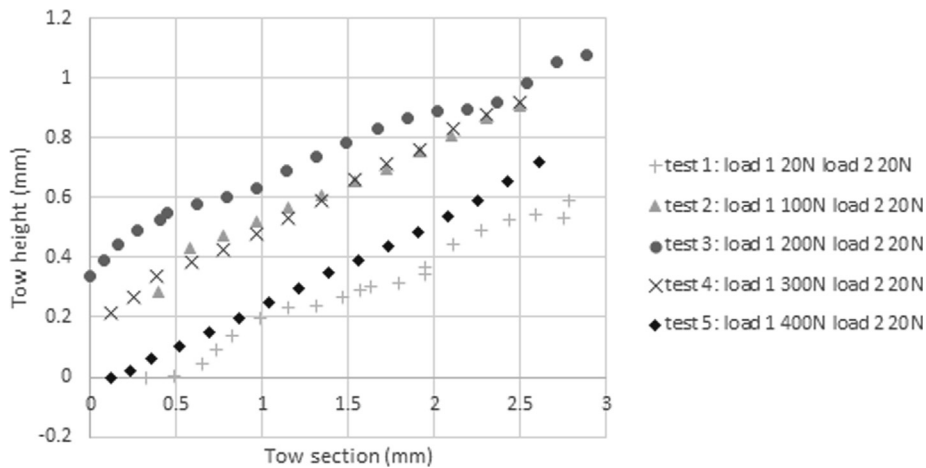
Fig. 11. Final sized up flax tow profiles under an in-plane bending angle of ~40°.
