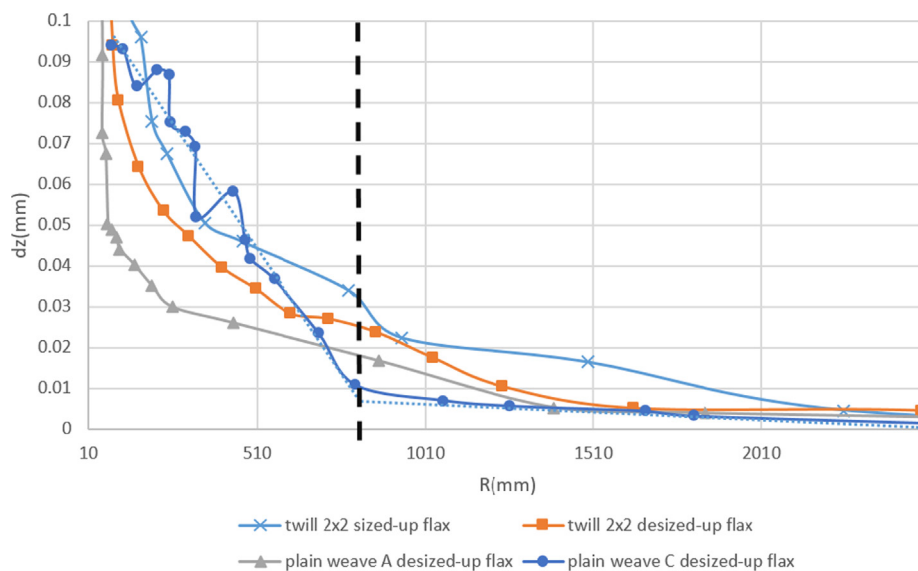
Fig. 19. Tow elevation evolution as a function of the bending radius. (For interpretation of the references to color in this figure legend, the reader is referred to the web version of this article.)
