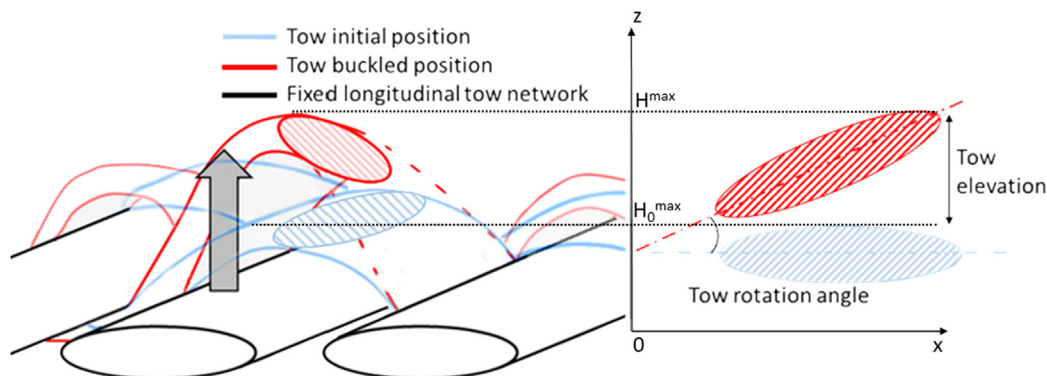
Fig. 5. Tow buckling illustration. (For interpretation of the references to color in this figure legend, the reader is referred to the web version of this article.)
