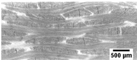
(yz) plane
