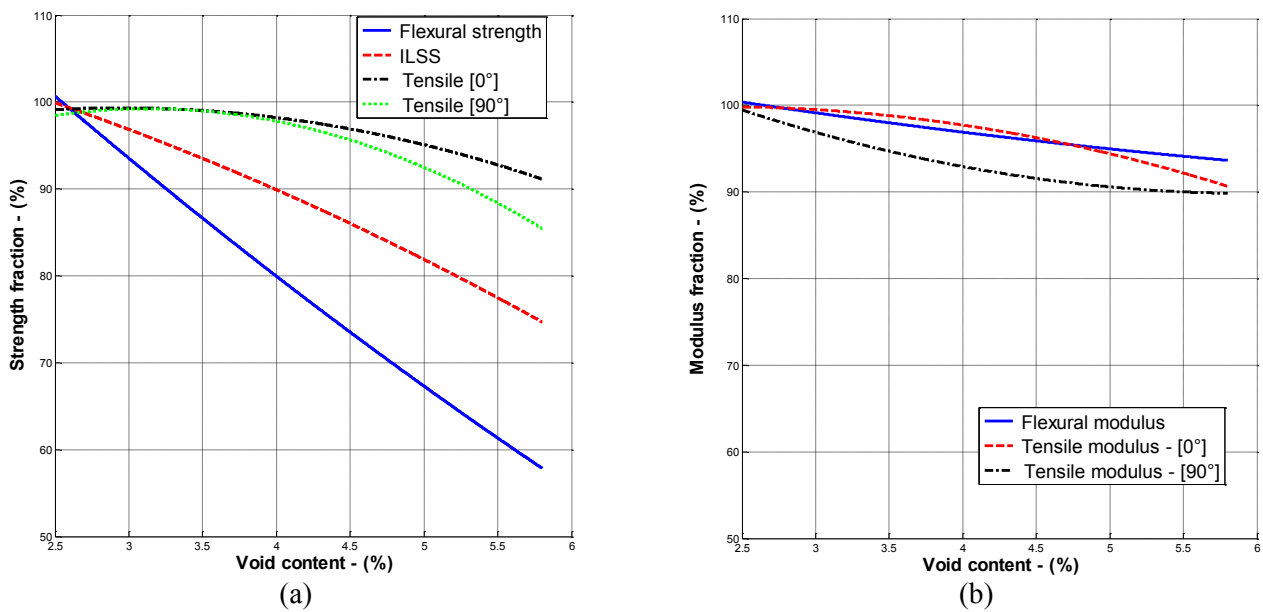
Figure 7. Relative mechanical properties variation : a) Strengths – b) Moduli
