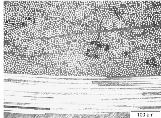
Figure 4. Micrograph of specimen N°3
