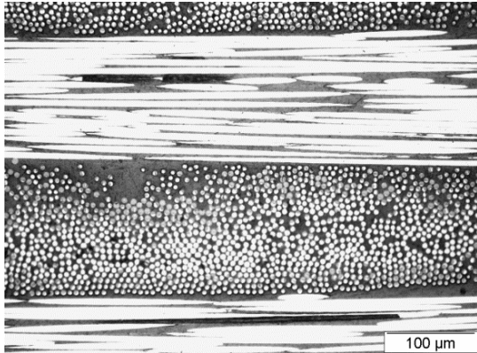
Figure 3. Micrograph of specimen N°2
