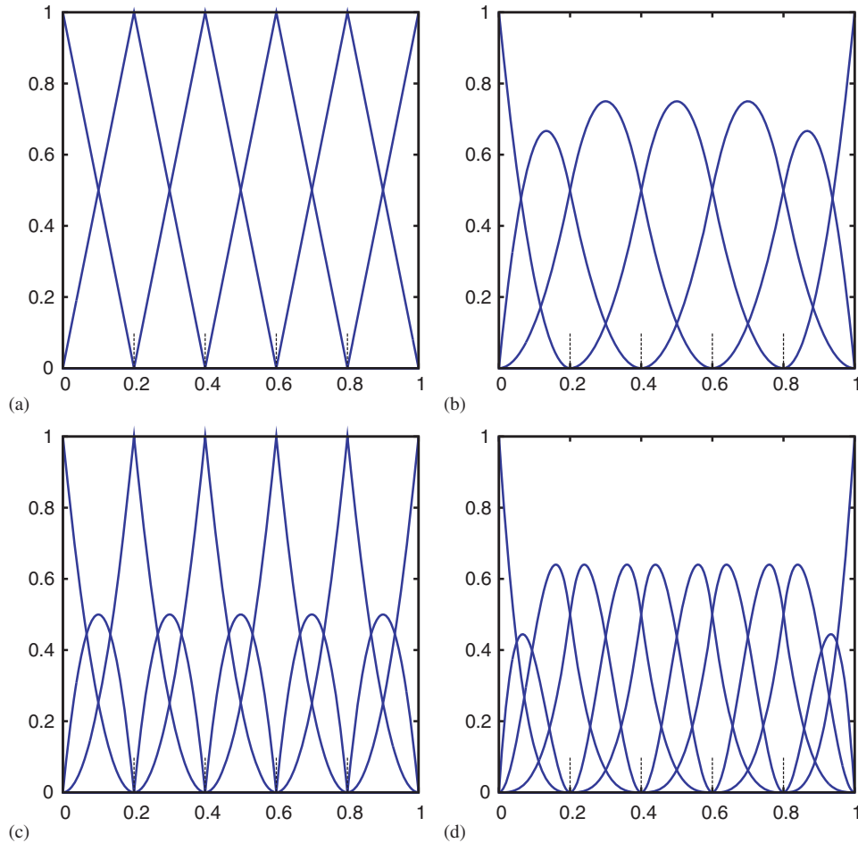
Figure 1. One-dimensional basis functions for 5 elements on the parametric domain. (a) \Xi=[0, 0, .2, .4, .6, .8, 1, 1] degree 1, multiplicity equal to 1; (b) \Xi=[0, 0, 0, .2, .4, .6, .8, 1, 1, 1] degree 2, multiplicity equal to 1; (c) \Xi=[0, 0, 0, .2, .2, .4, .4, .6, .6, .8, .8, 1, 1, 1] degree 2, multiplicity equal to 2; (d) \Xi=[0, 0, 0, 0, .2, .2, .4, .4, .6, .6, .8, .8, 1, 1, 1, 1] degree 3, multiplicity equal to 2.
