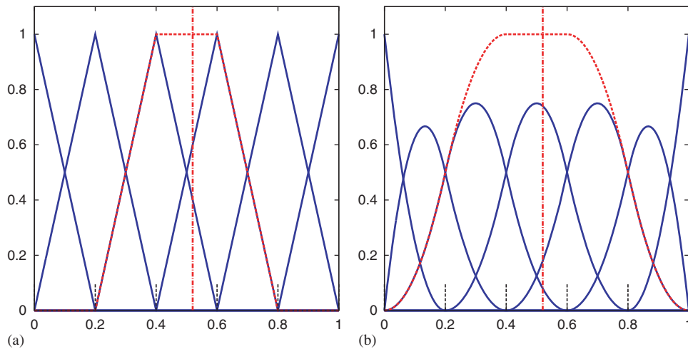
Figure 9. Enriched domain for 5 elements cut at x=0.45 . (a) Linear basis functions and (b) quadratic NURBS basis functions.
