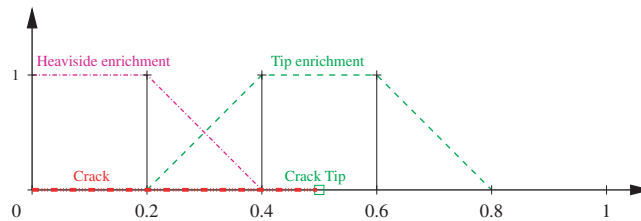
Figure 19. Linear blending functions for the Heaviside enrichment B_{\mathcal{H}} , and the tip enrichment B_{\mathcal{T}} .
