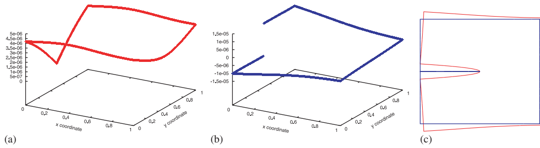
Figure 3. Displacement on the boundary of the domain for pure mode I and a stress-intensity factor K_1=100 . (a) X displacement; (b) Y displacement; and (c) magnified deformation
