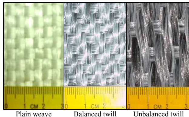
Fig. 1. Woven fabrics
