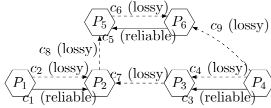
Figure 5.5: A topology that splits in three
