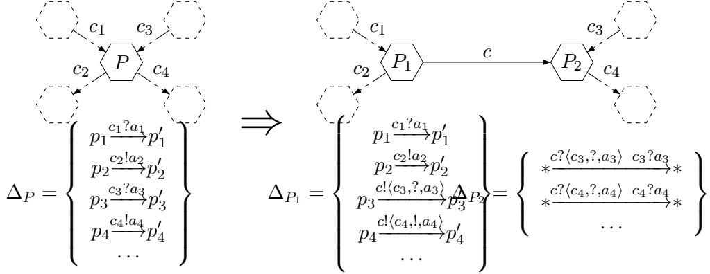
Figure 5.4: Associating a T -MCS with a T/c -MCS
