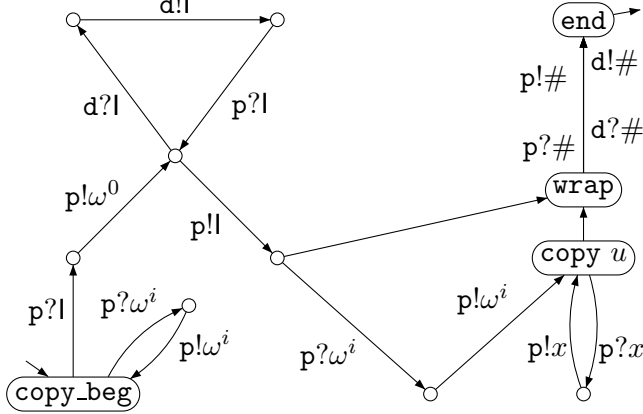
Figure 3.6: LCS component that implements rule S2 (assuming purity)
